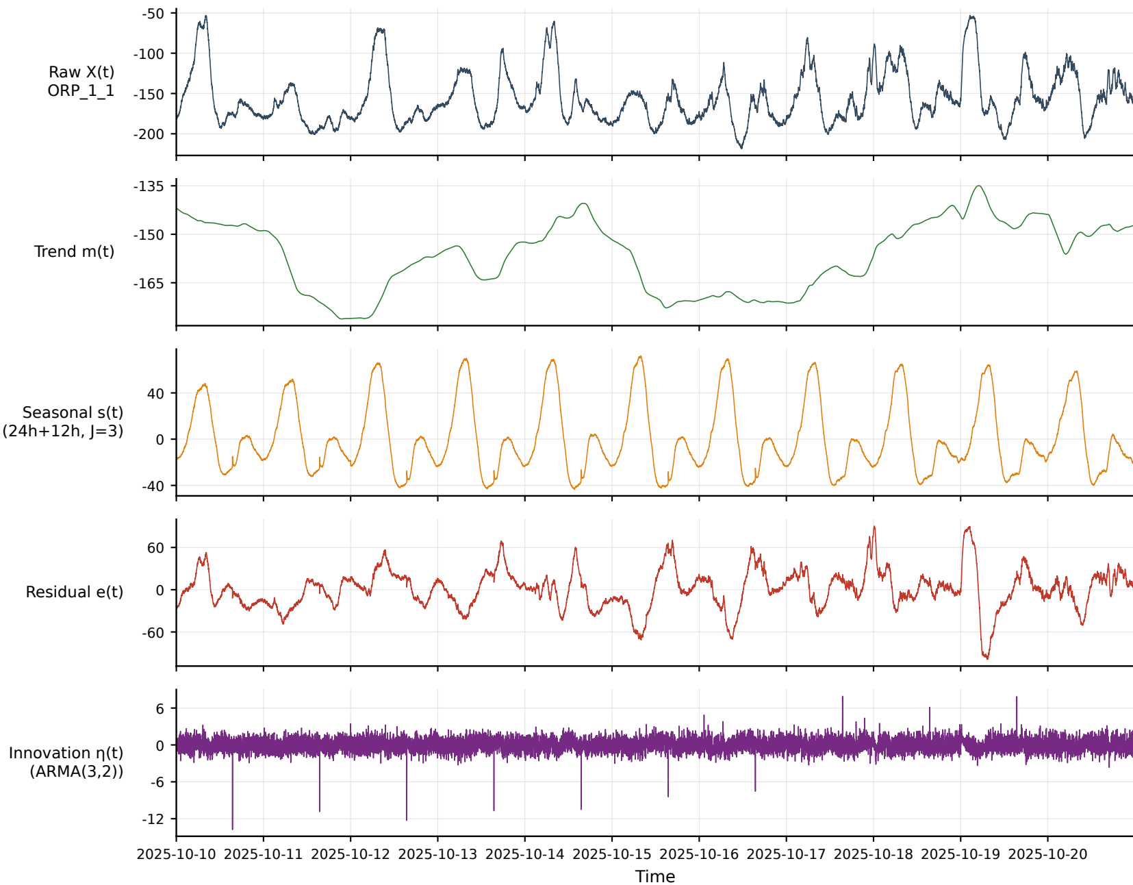
Multi-scale decomposition — ORP_1_1 (anaerobic, min) [2025-10-10~2025-10-20]
